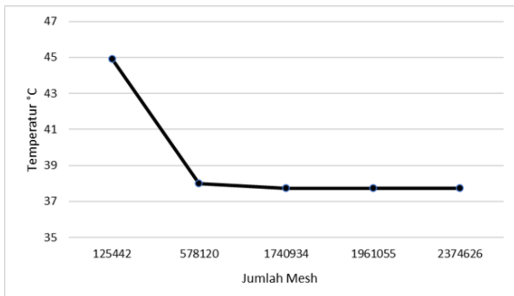
GAMBAR 6. Mesh Independence Test.
