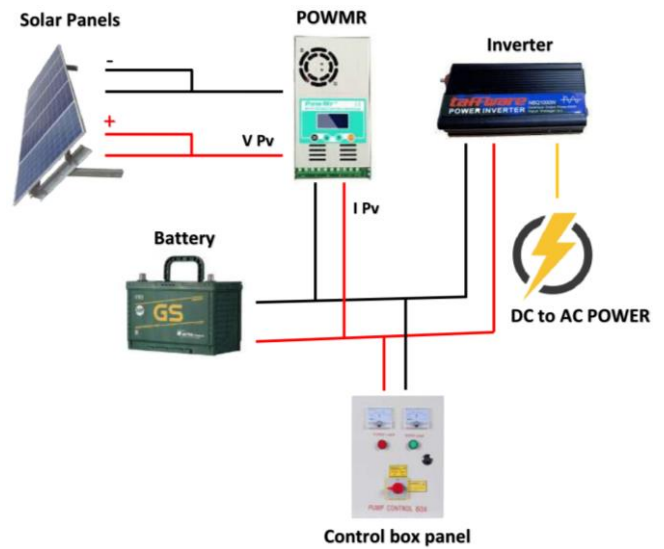
Fig. 5 PLTS wiring power system.
