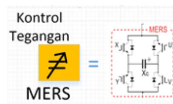
Gbr. 1 Kontrol tegangan MERS.
