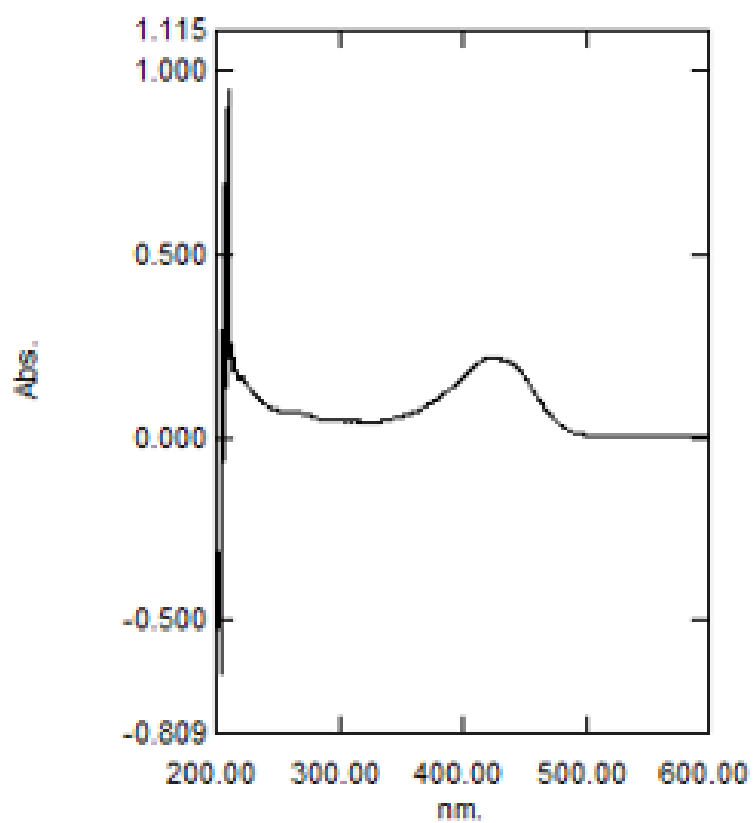
Supplementary Figure 1. HPLC (A) and UV-Vis (B) analysis of isolate 1.
