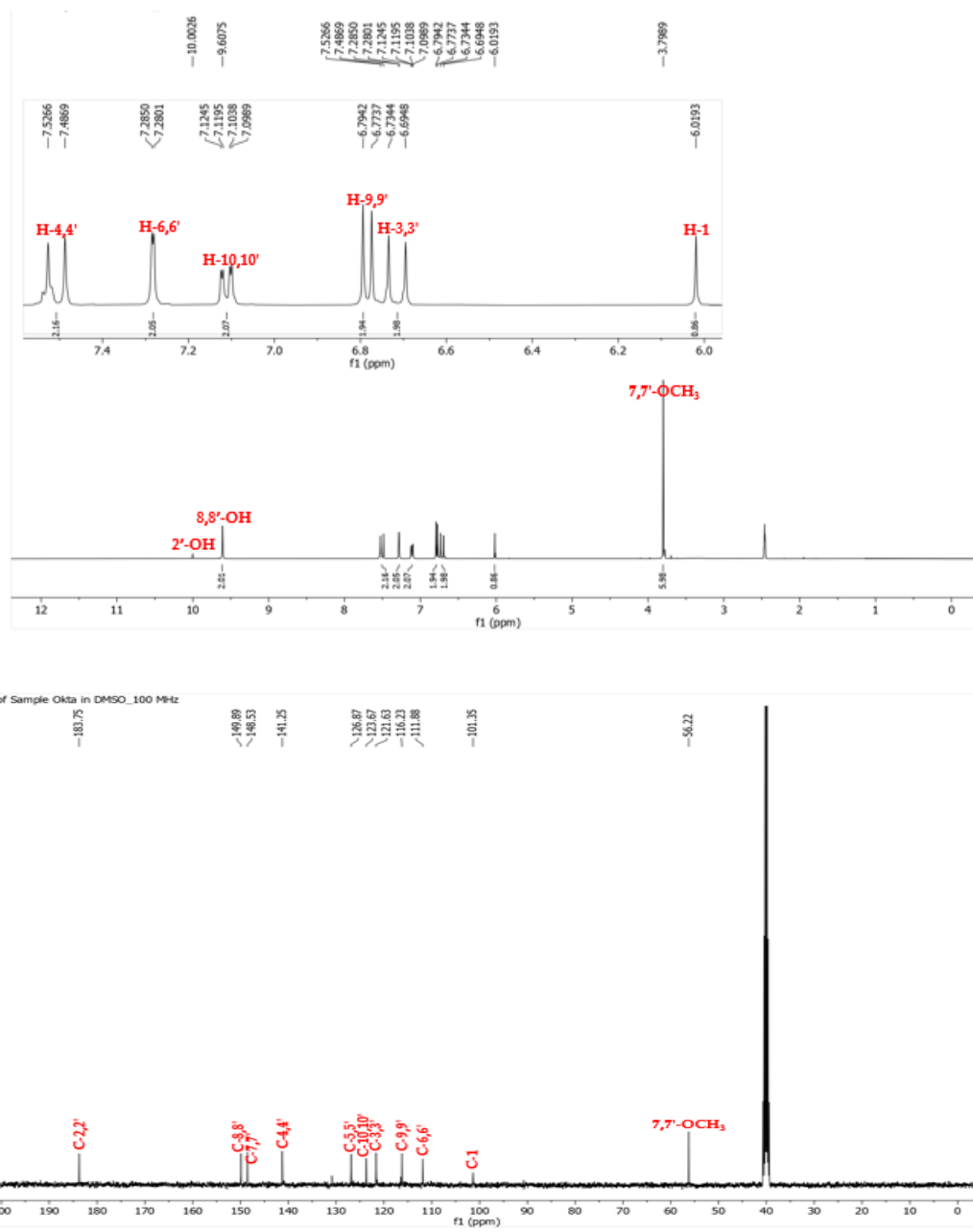
Supplementary Figure 3. NMR analysis of isolate 1. Analysis ^1\text{H} -NMR (A) and ^{13}\text{C} -NMR (B) analysis.
