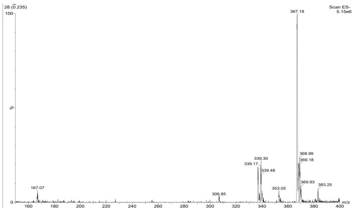
Supplementary Figure 2. FTIR (A) and Mass Chromatography (B) analysis of isolate 1.
