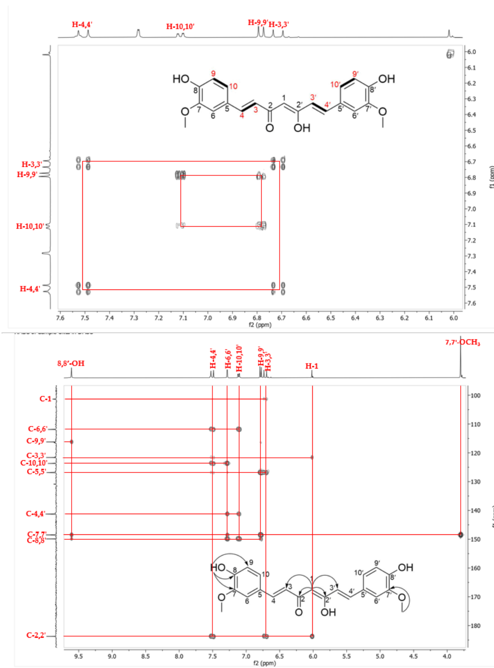
Supplementary Figure 4. 2D-NMR analysis of isolate 1. Analysis COSY (A) and HMBC (B) analysis.
