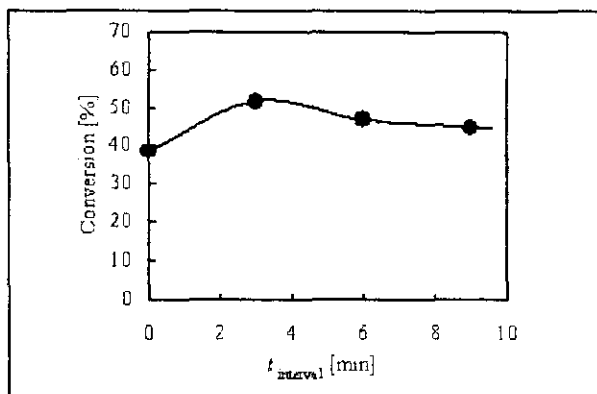
Figure 11. Effect of Pulse Interval on Conversion at T=110^{\circ}\text{C} , Ru-Pt/C, and 62\mu\text{mol/s}
