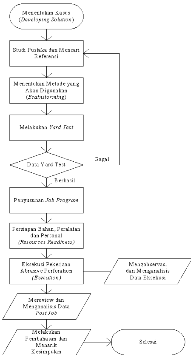
GAMBAR 2. Diagram alir kegiatan abrasive perforation
