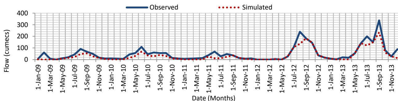
Figure 9. Comparison of observed and simulated flow discharge (at SW266 station) during validation period (2009 – 2013)
