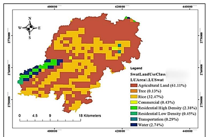
Figure 5. Land use map of Surma basin
