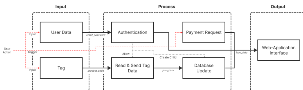
Gambar 2.3 Diagram Input-Proses-Output
