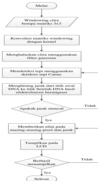
Gambar 3 Alur Gaussian Filter
