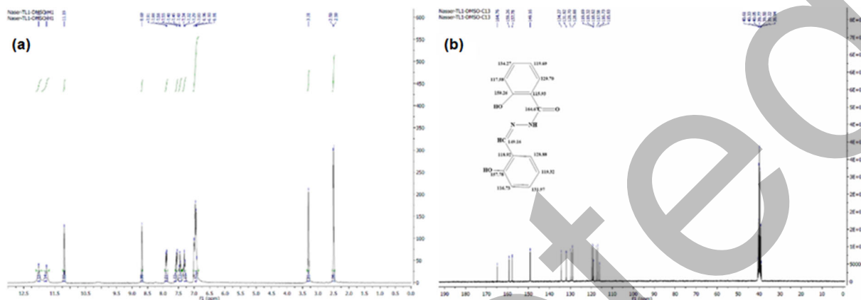
Fig S1. (a) ^1\text{H-NMR} and (b) ^{13}\text{C-NMR} of LH
