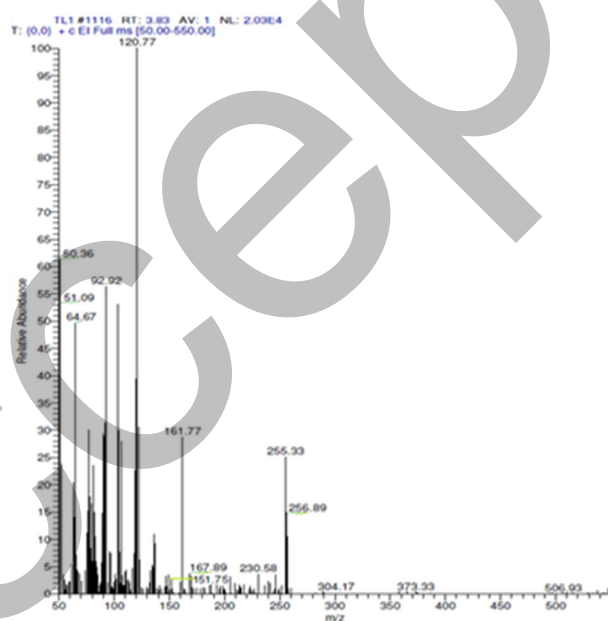
Fig S2. Mass spectrum of LH
