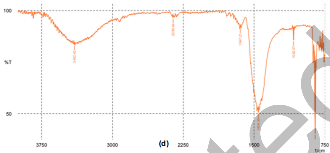
Fig S1. FTIR peak patterns of PCC synthesized under different conditions: (a) \text{NH}_4\text{Cl} 75 g/L at 30 °C, (b) \text{NH}_4\text{Cl} 50 g/L at 55 °C, (c) \text{NH}_4\text{Cl} 75 g/L at 55 °C, and (d) \text{NH}_4\text{Cl} 50 g/L at 30 °C
