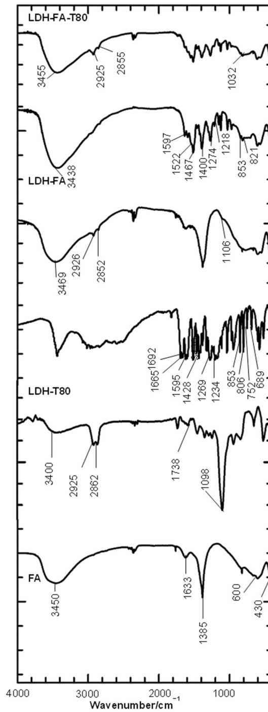
Fig S1. FTIR spectra of LDH, Tween-80, FA, LDH-T80, LDH-FA, and LDH-FA-T80 nanocomposites
