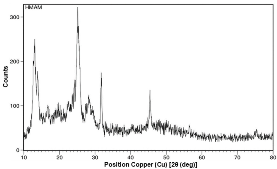
Fig S5. X-ray diffraction of SBDP-DMP ligand
