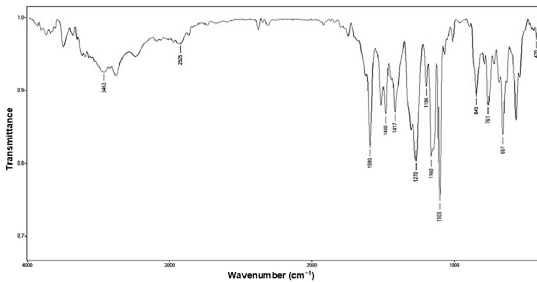
Fig S2. Infrared spectrum of SBDP-DMP ligand
