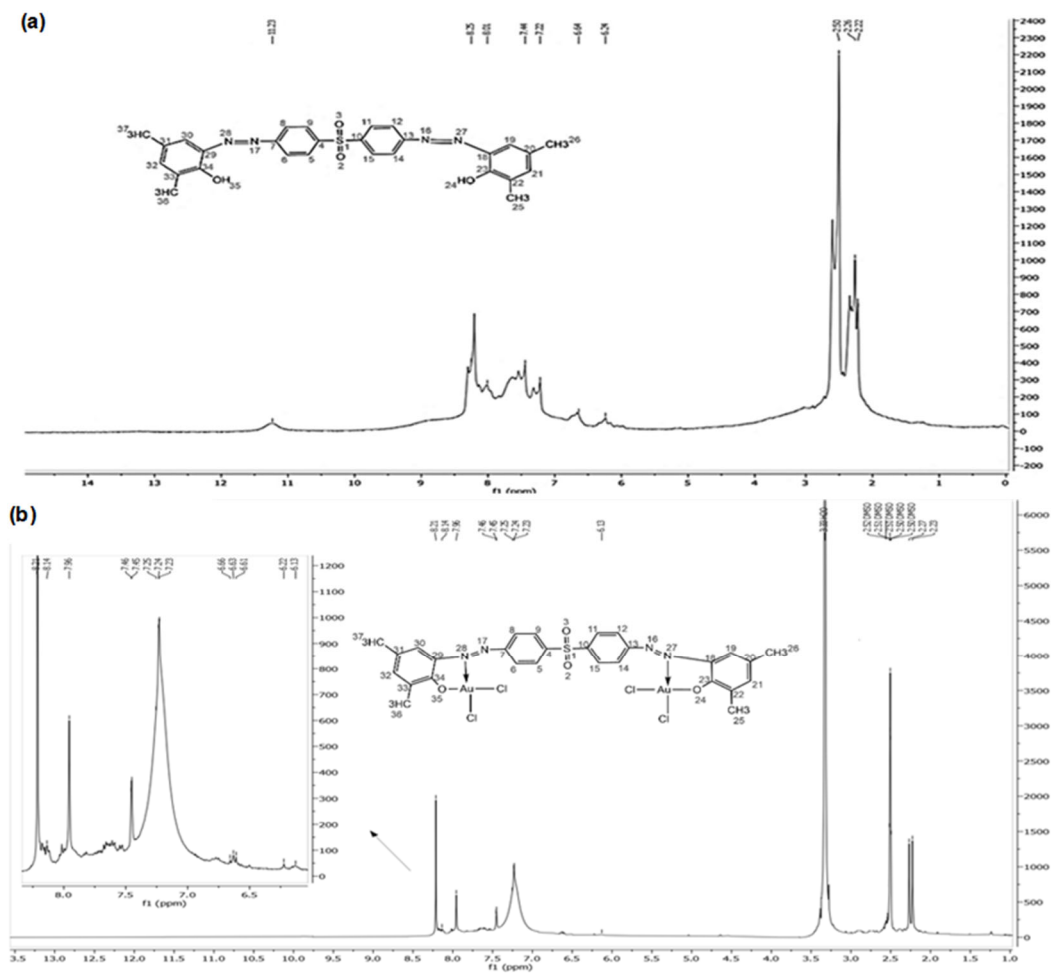
Fig S1. 1 H-NMR spectrum of (a) SBDP-DMP ligand and (b) its Au(III) complex in DMSO- d 6 solvent
