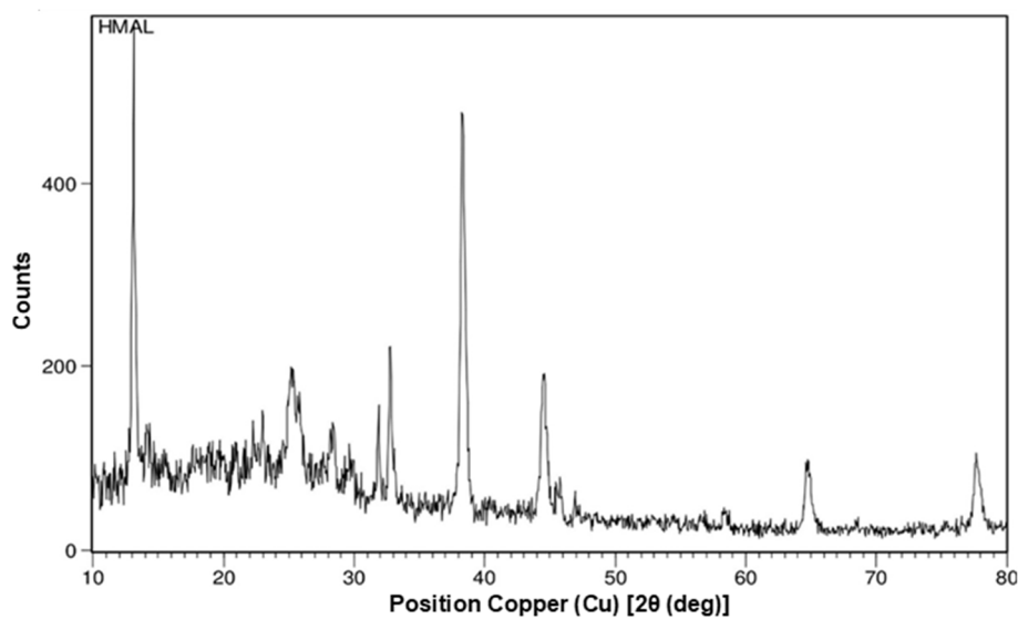
Fig S6. X-ray diffraction of Au(III) complex with SBDP-DMP ligand
