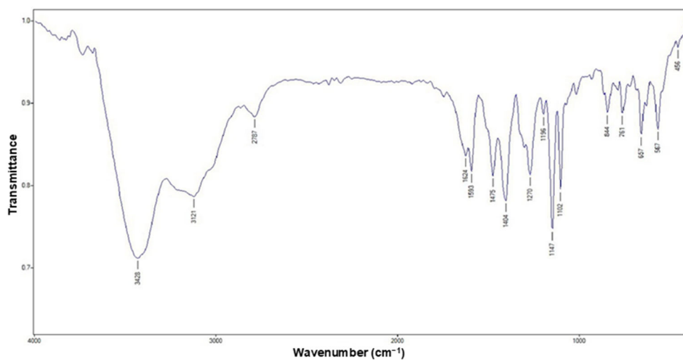
Fig S3. Infrared spectrum of Au(III) complex with SBDP-DMP ligand
