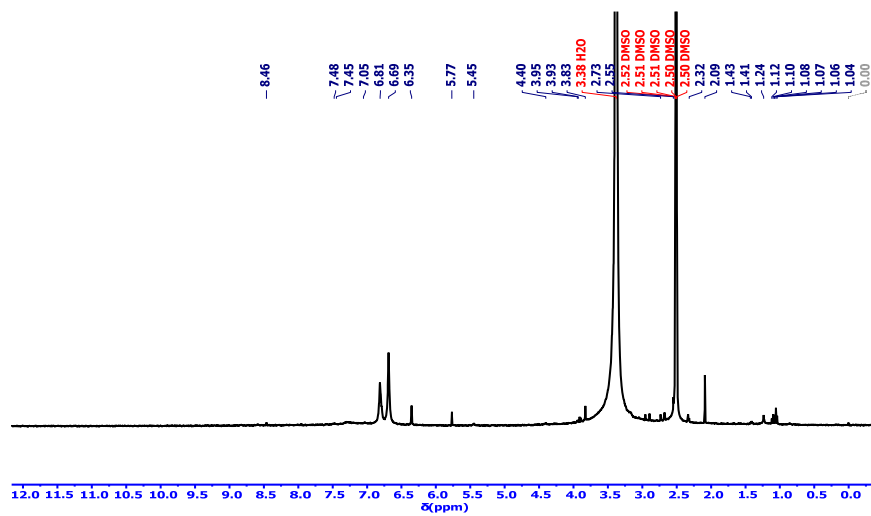
Fig S16. 1 H-NMR spectrum of compound VII
