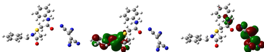
Fig S26. Molecular structure and molecular orbitals (HOMO and LUMO) of compound VI
