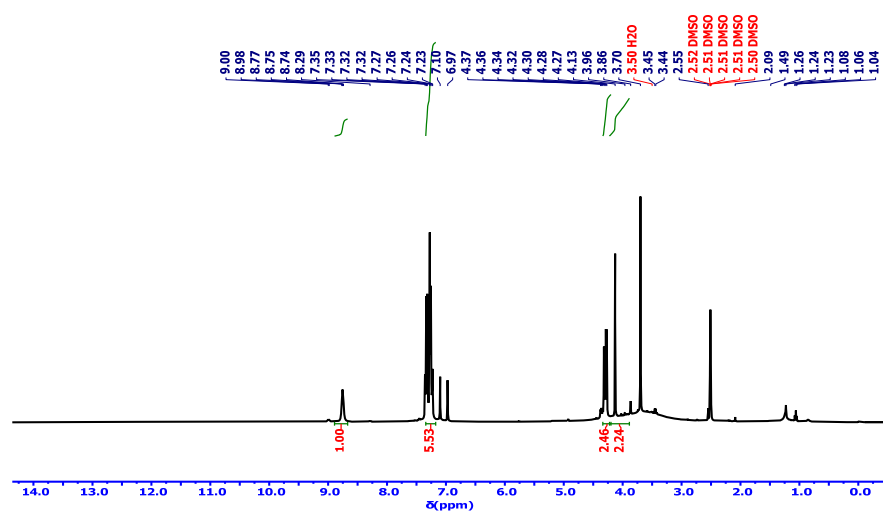
Fig S12. 1 H-NMR spectrum of compound III
