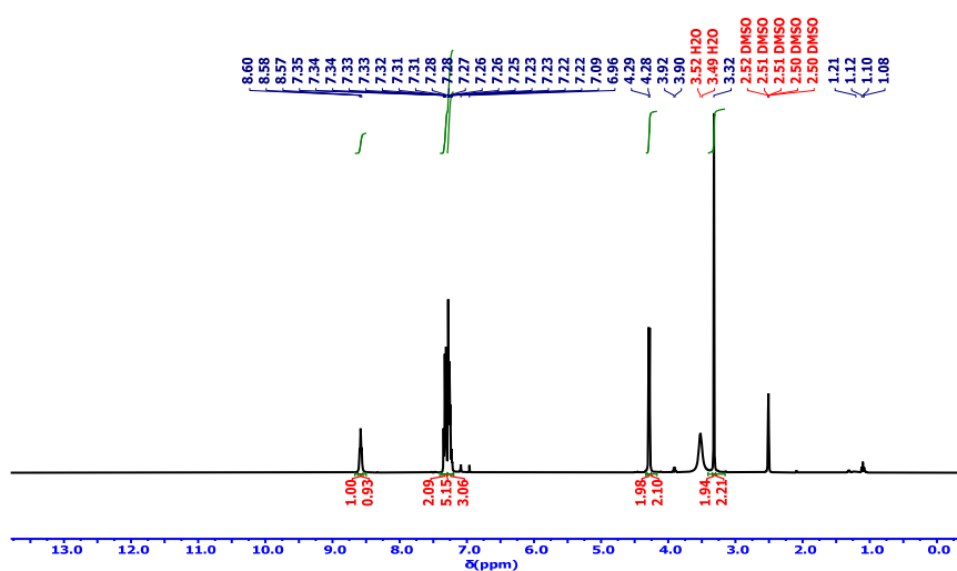
Fig S15. 1 H-NMR spectrum of compound VI
