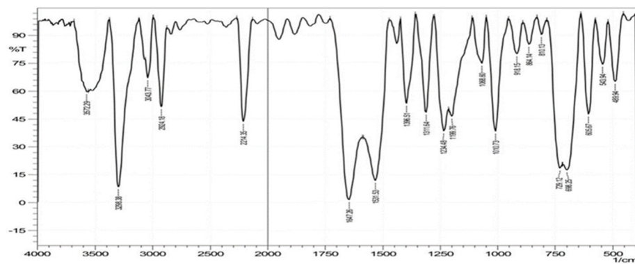
Fig S6. Infrared spectrum of compound VI
