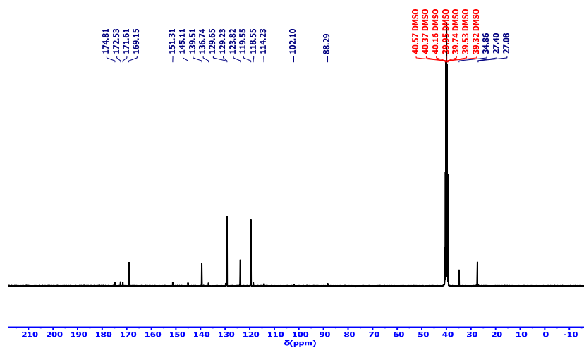
Fig S20. ^{13}\text{C-NMR} spectrum of compound IV
