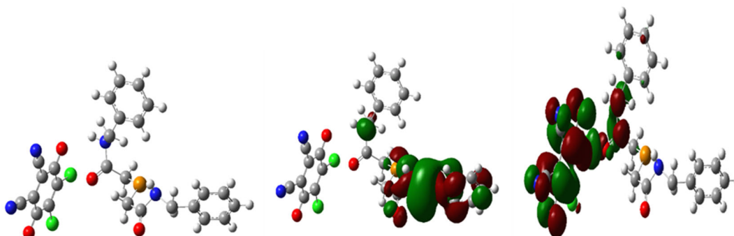
Fig S25. Molecular structure and molecular orbitals (HOMO and LUMO) of compound III
