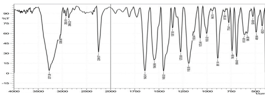
Fig S2. Infrared spectrum of compound II
