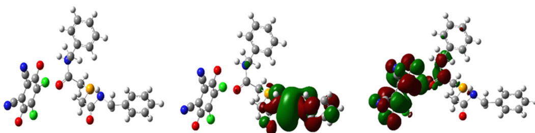
Fig S24. Molecular structure and molecular orbitals (HOMO and LUMO) of compound II
