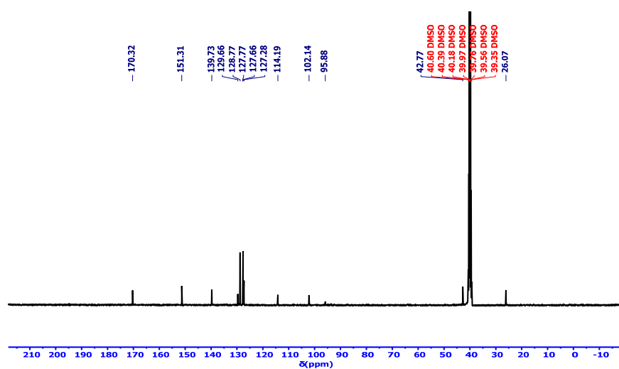
Fig S18. 13 C-NMR spectrum of compound II
