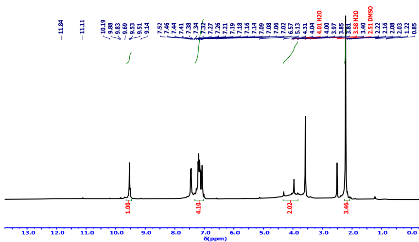
Fig S14. 1 H-NMR spectrum of compound V
