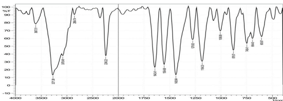
Fig S3. Infrared spectrum of compound III
