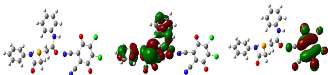
Fig S29. Molecular structure and molecular orbitals (HOMO and LUMO) of compound IV
