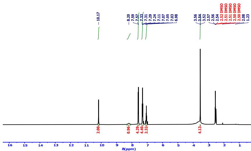
Fig S13. 1 H-NMR spectrum of compound IV
