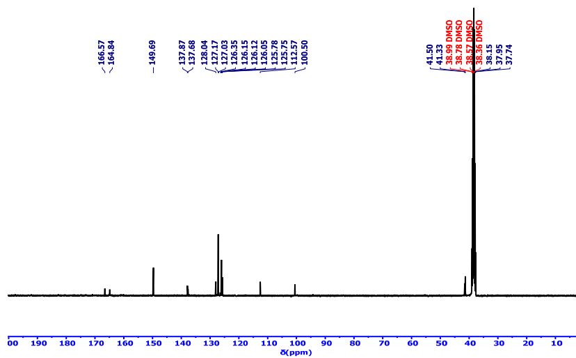
Fig S19. ^{13}\text{C-NMR} spectrum of compound III
