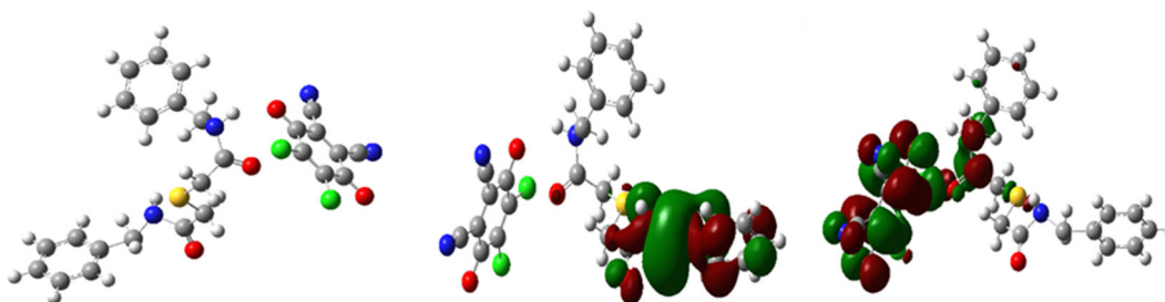
Fig S23. Molecular structure and molecular orbitals (HOMO and LUMO) of compound I
