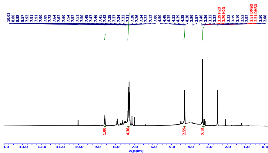
Fig S10. 1 H-NMR spectrum of compound I
