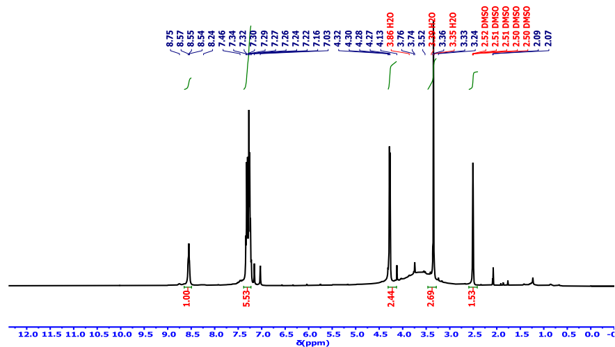
Fig S11. 1 H-NMR spectrum of compound II
