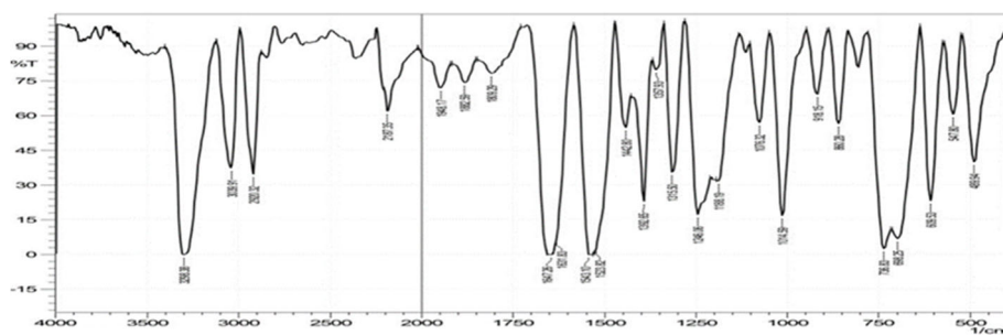
Fig S8. Infrared spectrum of compound VIII
