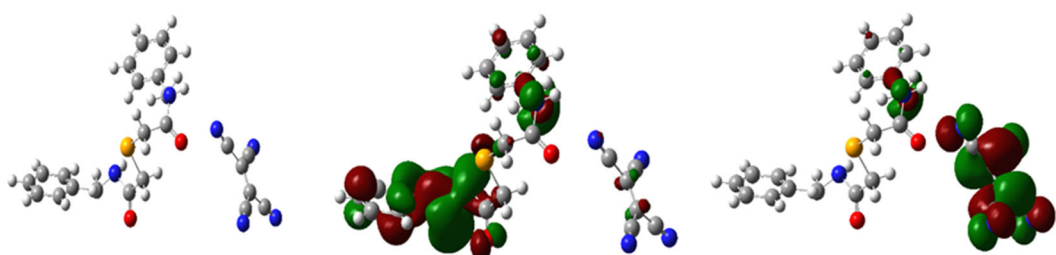
Fig S27. Molecular structure and molecular orbitals (HOMO and LUMO) of compound VII
