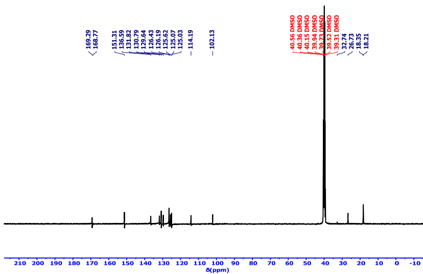
Fig S21. ^{13}\text{C-NMR} spectrum of compound V
