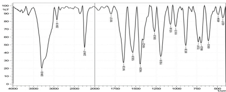
Fig S1. Infrared spectrum of compound I
