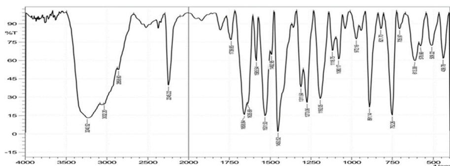
Fig S5. Infrared spectrum of compound V
