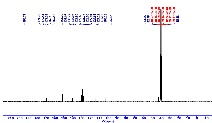
Fig S17. 13 C-NMR spectrum of compound I
