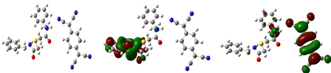
Fig S28. Molecular structure and molecular orbitals (HOMO and LUMO) of compound VIII
