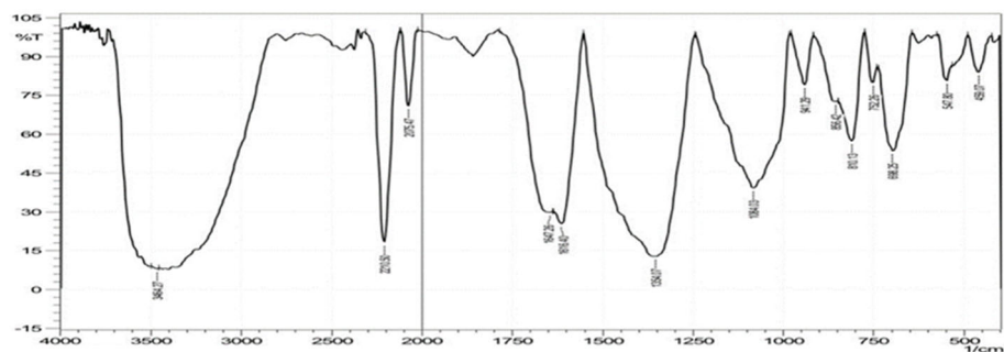
Fig S7. Infrared spectrum of compound VII
