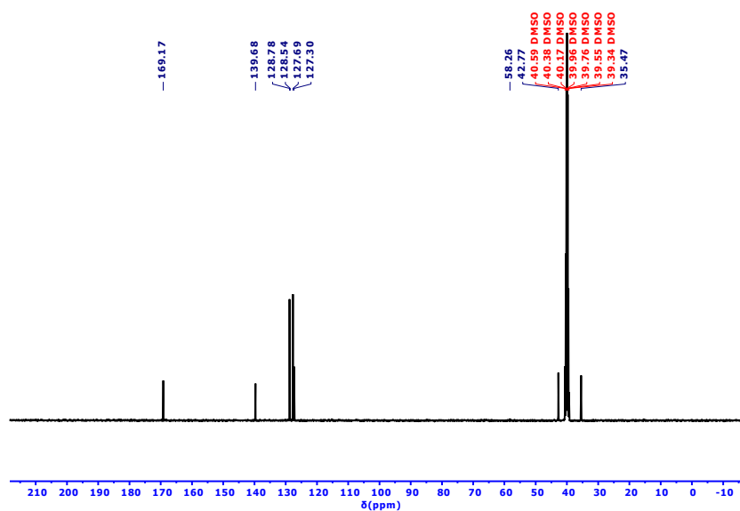
Fig S22. ^{13}\text{C} -NMR spectrum of compound VI
