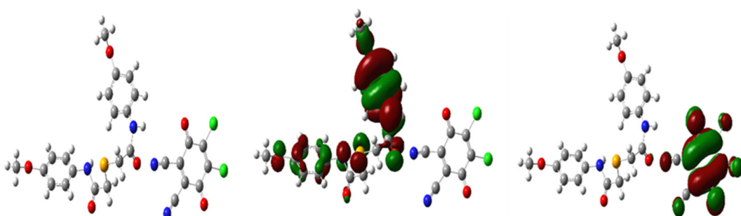
Fig S30. Molecular structure and molecular orbitals (HOMO and LUMO) of compound V
