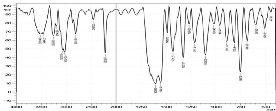
Fig S4. Infrared spectrum of compound IV
