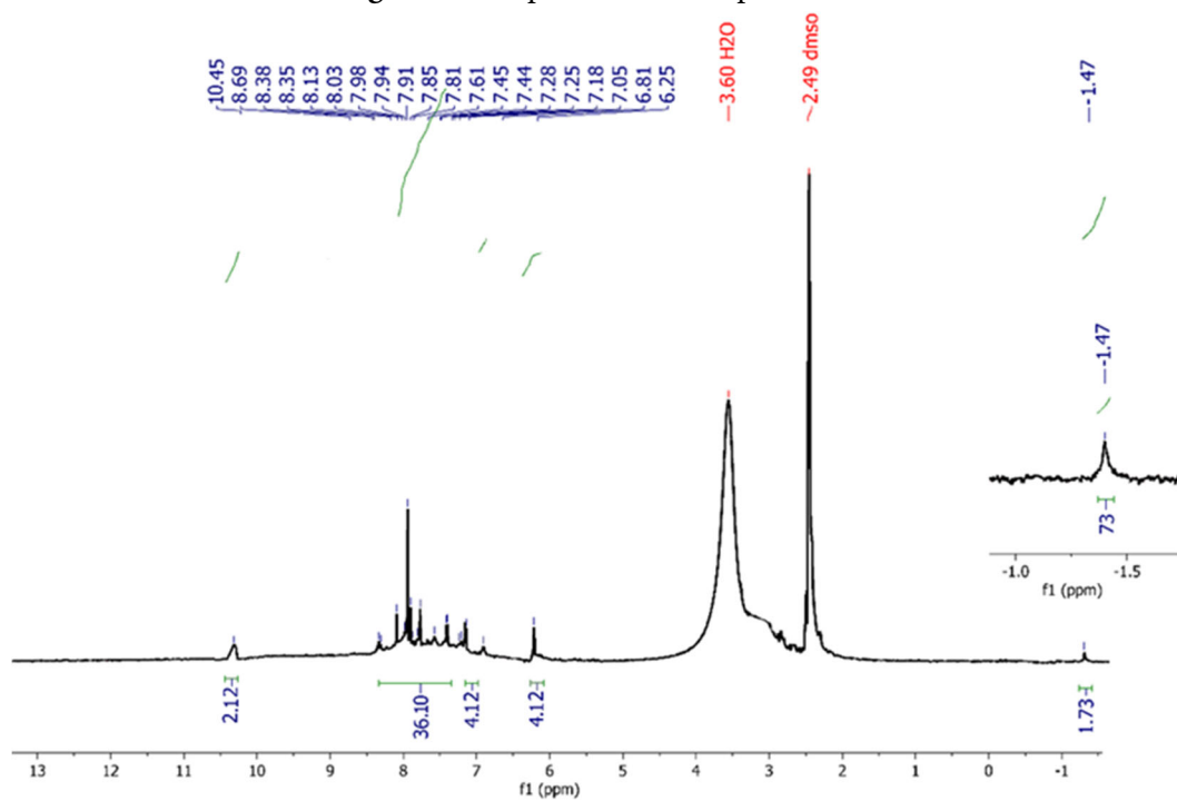
Fig S8. 1 H-NMR spectrum of compound 5a
