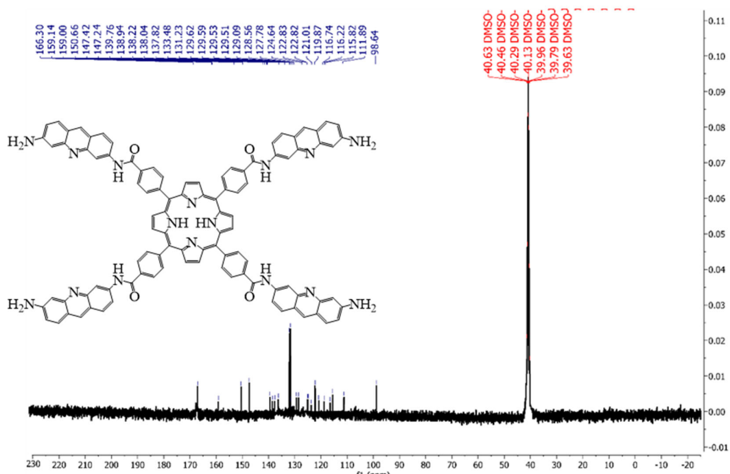
Fig S5. 13 C-NMR spectrum of compound 3a
