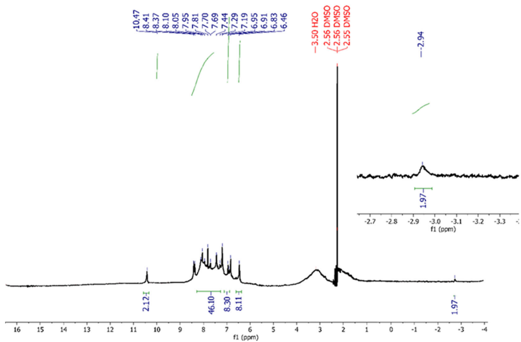
Fig S3. 1 H-NMR spectrum of compound 3a
