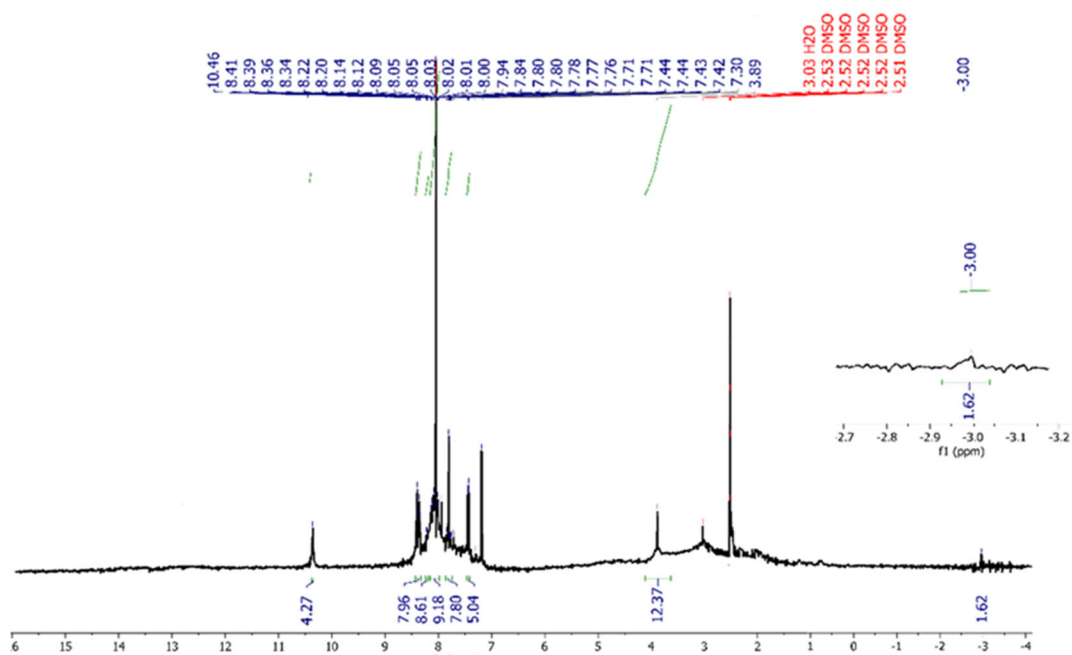
Fig S4. 1 H-NMR spectrum of compound 3b
