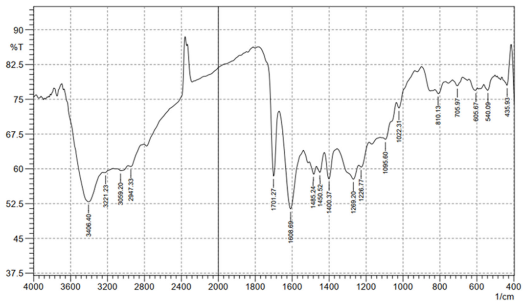
Fig S7. FTIR spectrum of compound 5b
