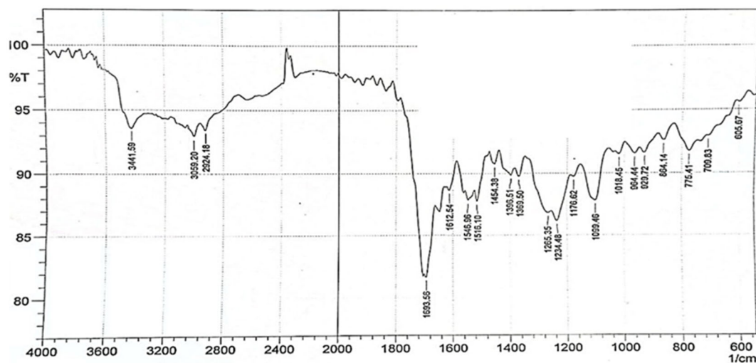
Fig S2. FTIR spectrum of compound 3b
