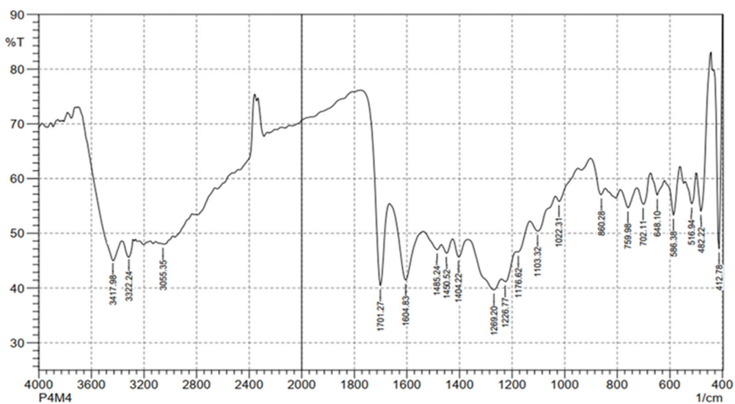
Fig S6. FTIR spectrum of compound 5a
