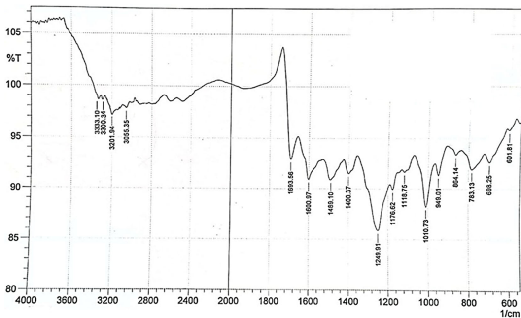
Fig S1. FTIR spectrum of compound 3a
