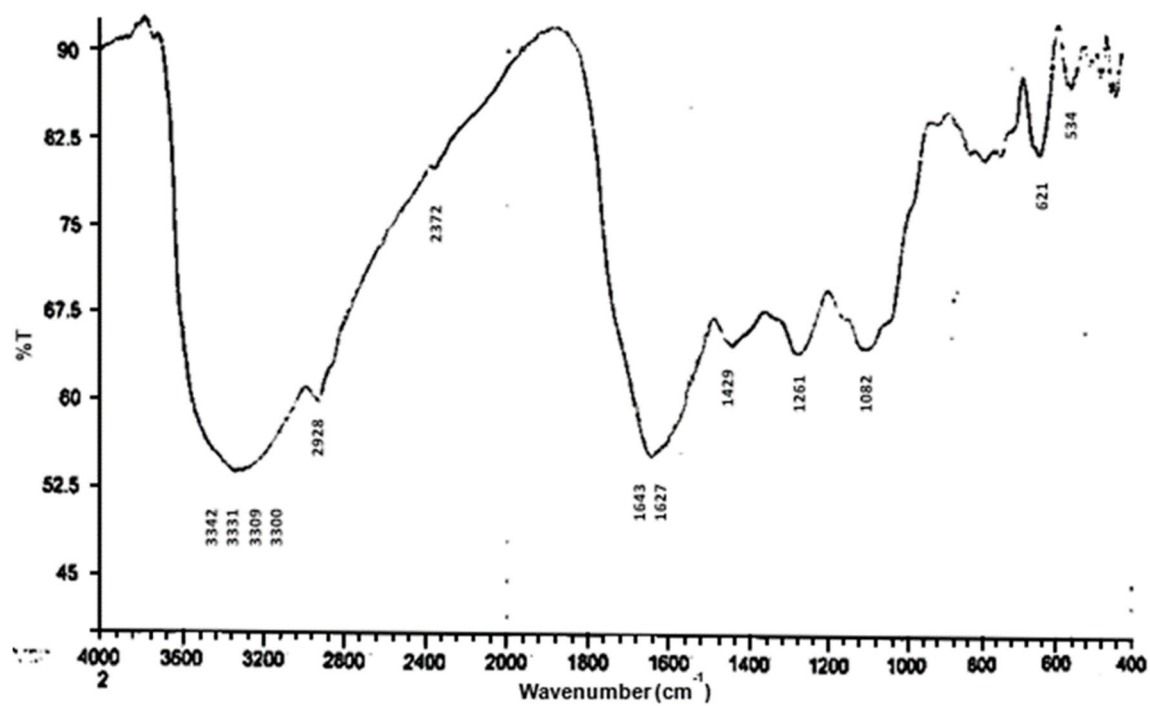
Fig S1. FTIR spectrum of nano-copper
