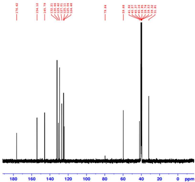
Fig S2. ^{13}\text{C-NMR} spectrum of ligand L
