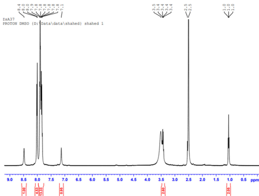
Fig S1. ^1\text{H-NMR} of 1,2,4-triazole (L)
