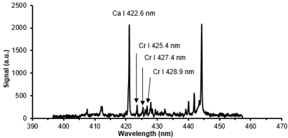
Fig 9. Emission spectrum taken from the agar powder containing 1% Cr using the mesh-assisted laser-induced plasma spectroscopy employing confinement technique
