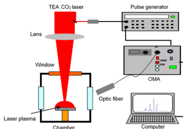
Fig 1. Experimental setup used in this work
