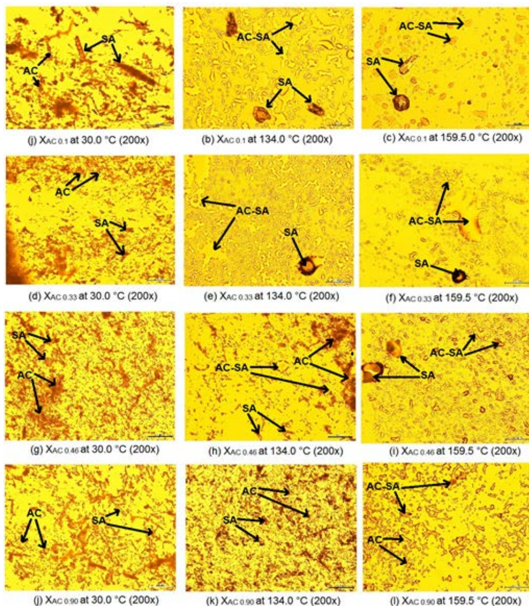
Fig 5. Thermomicroscopy of binary mixtures of AC-SA
