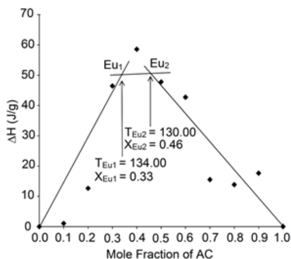
Fig 3. Tamman diagram of binary mixtures of AC-SA
