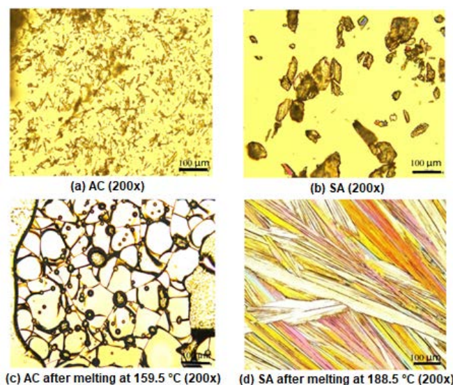
Fig 4. Microstructure of AC and SA after melting
