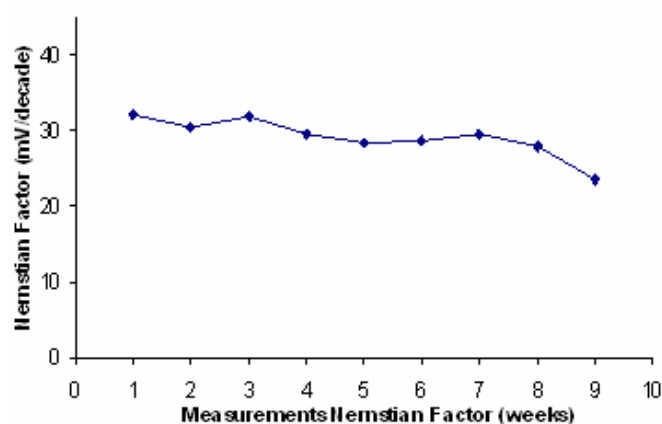
Fig 6. Nernstian factor value changes from ESI \text{Cd}^{2+} for every weeks
