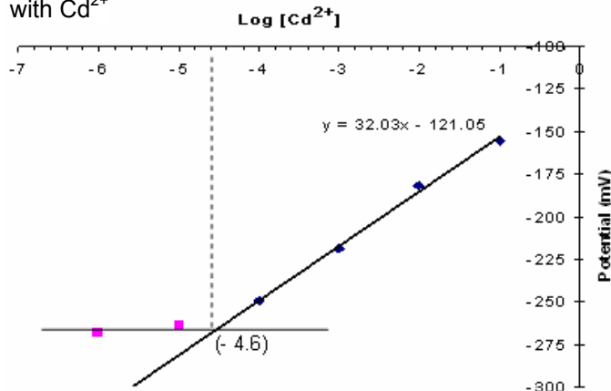
Fig 4. Determination of Nernstian factor and Detection limit of ISE Cd 2+
