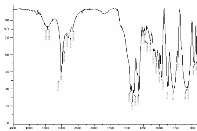
Fig 3. FT-IR spectra Chitosan Membranes after doped with Cd 2+
