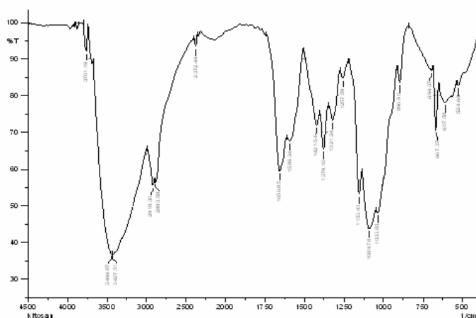
Fig 2. FT-IR spectra Chitosan Membrane before doped with Cd 2+
