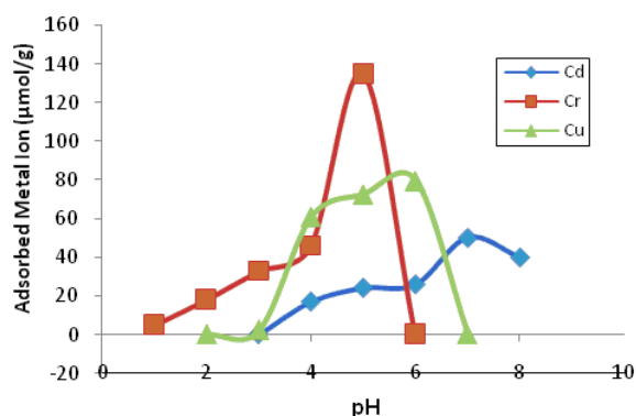
Fig 2. Effect of pH on adsorption of Cd(II), Cu(II) and Cr(III) onto polymer 2a
