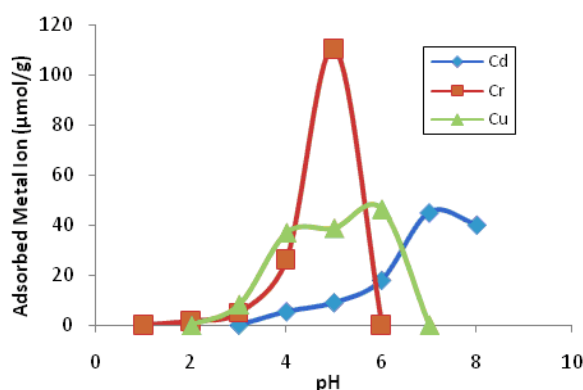
Fig 3. Effect of pH on adsorption of Cd(II), Cu(II) and Cr(III) onto polymer 2b
