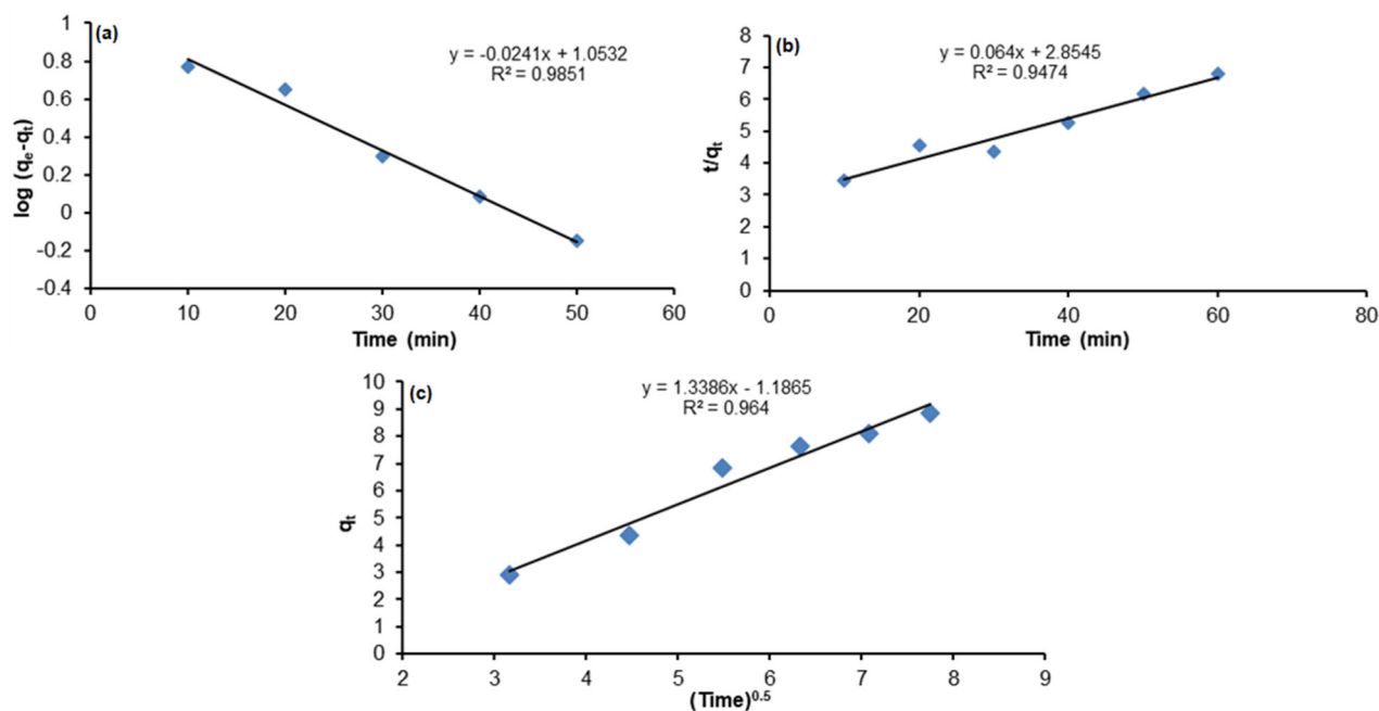
Fig S2. Kinetics models of adsorption of MB adsorption on Si-Zn NC, (a) pseudo-first-order, (b) pseudo-second-order, and (c) intra particle diffusion
