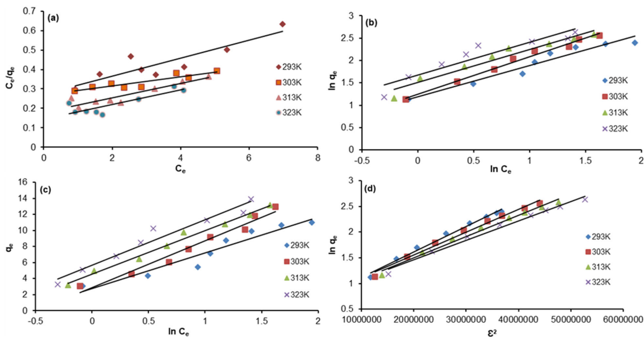
Fig S1. Linear relation of isotherms (a) Langmuir, (b) Freundlich, (c) Temkin, and (d) Dubinin-Radushkevich models of MB adsorption on Si-Zn NC
