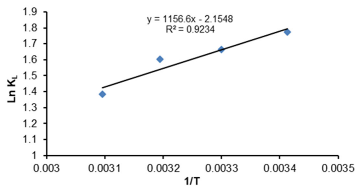
Fig S3. The van't Hoff plot of MB adsorption onto Si-Zn NC
