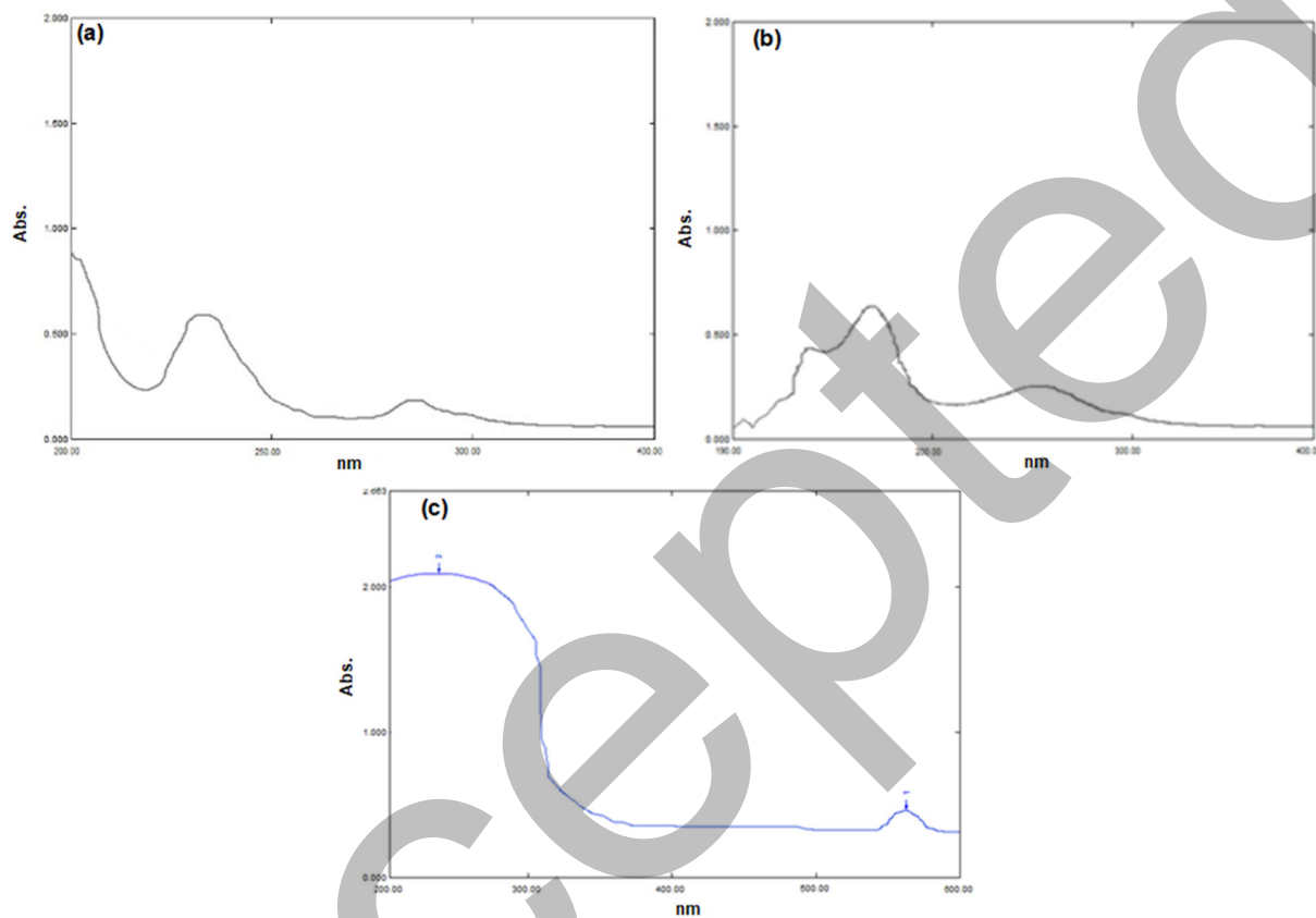
Fig S1. UV-vis spectra of (a) L1, (b) AL1, and (c) AL2
