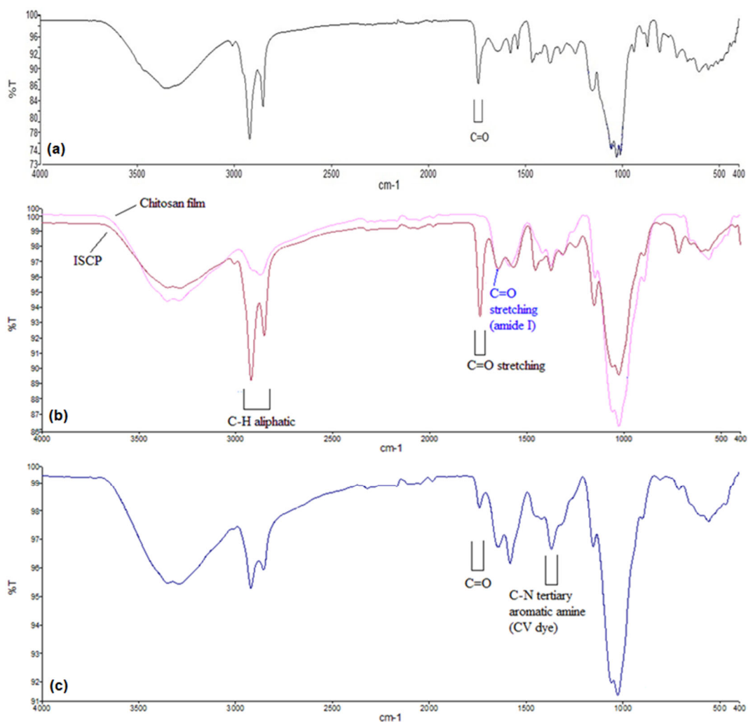
Fig S1. ATR-FTIR spectra of (a) SCP, (b) chitosan film and ISCP, and (c) ISCP after the adsorption of CV dye
