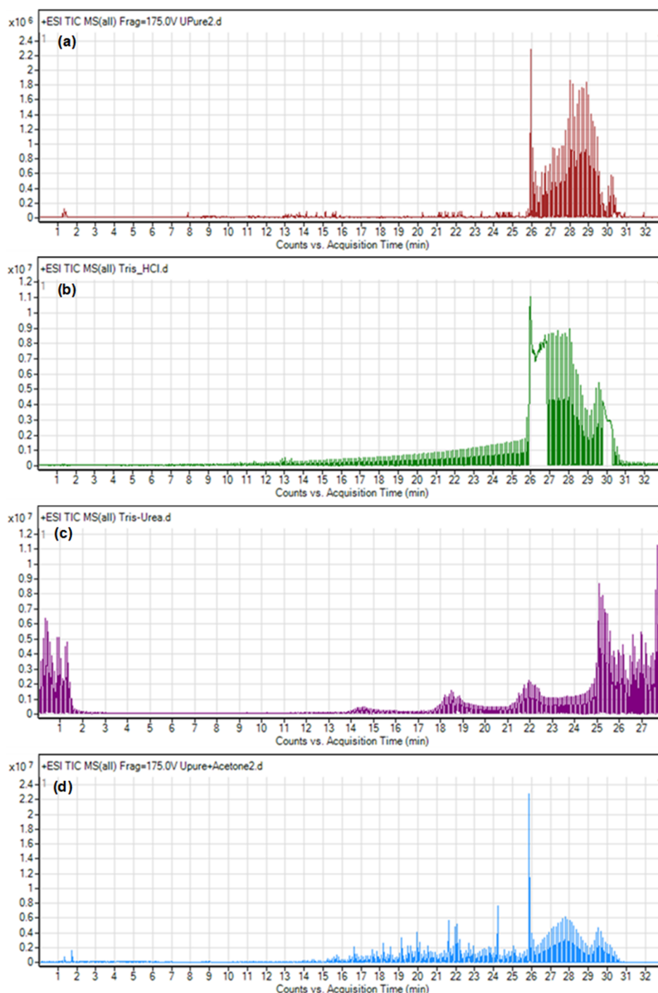
Fig S1. TIC of CBP in different extraction buffers (a) ultrapure water, (b) 0.05 M Tris-HCl, (c) 0.05 M Tris-Urea, and (d) ultrapure water with acetone
