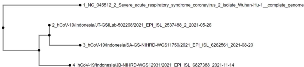
FIGURE 5 Phylogenetic tree of chosen Delta variant SARS-CoV-2 Indonesian isolates with the NC_045512.2 as reference.
