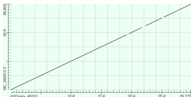
FIGURE 4 The nucleotide similarity range of Wuhan SARS-CoV-2 Wild-Type Isolate (NC_045512.2 from NCBI) vs an Indonesian Delta Variant Sample (EPI_ISL_2537488.2 from GISAID) obtained from NCBI BLAST.
