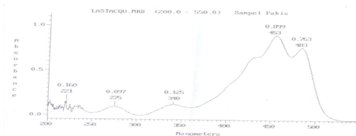
Gambar 7. Spektra visibel (CHCl 3 ) isolat batang Alsophila glauca J.Sm
