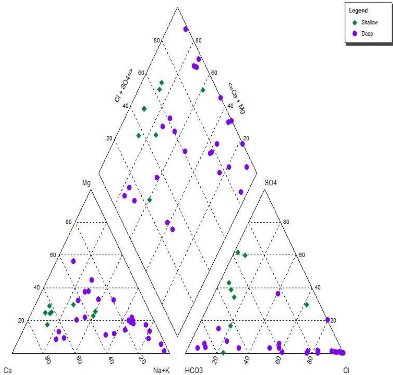
Figure 4. Piper diagram of the groundwater samples.
